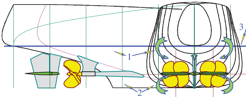
Figure 7 Aft valance, quarter, bottom bilge and stern-post of twin-screw ship, optimized to minimal trim on calm water way
