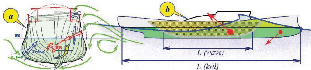
Figure 3 The hull form must given the hydrodynamic compensation: a – a rolling using by minimizing height of tumblehome board in the middle, and: b – pitching of ship through the redistribution of pressures in trochoidal wave on board.
