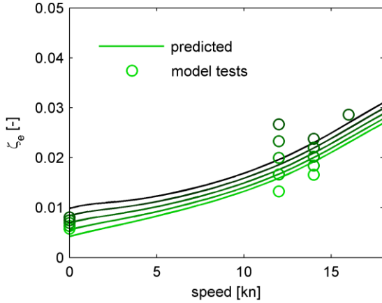
Figure 2: Predicted damping for the bare hull of a Pure Car and Truck Carrier in model scale using Ikeda's method with the lift damping component is estimated with hull lift coefficient from non-viscous CFD together with Yomuru's original expressions for the levers of the lift force and the effective angle of attack, compared with model tests for roll amplitudes of 2 to 10°.
