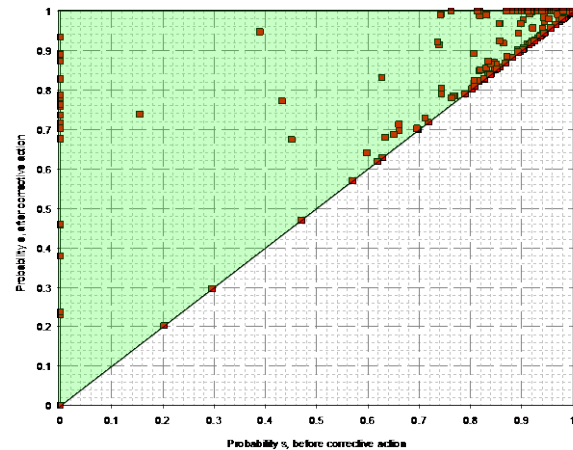
Fig. 4: Counter-balling capacity post-casualty (typical example)
