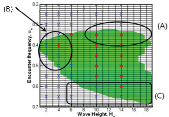
Fig. 3: Categorization of susceptible region of parametric roll
