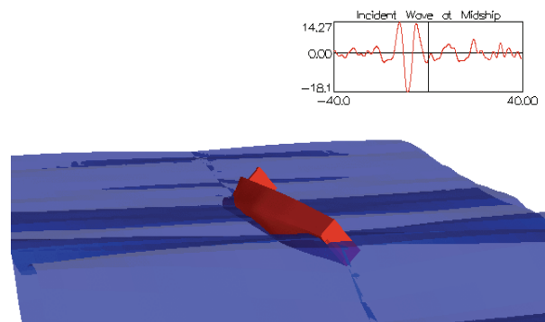
Fig. 6: Example LAMP Simulation (One of Three Capsizing Cases)
